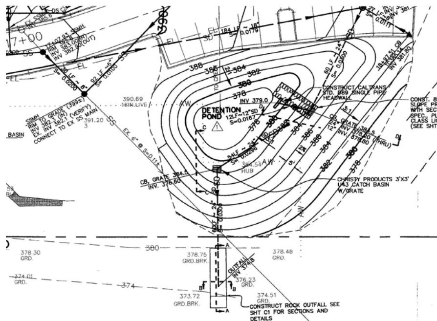
Design drawing of detention pond
